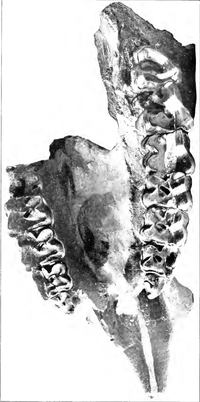
PALATE OF DICERATHERIUM ARMATUM MARSH U.S.N.M. No. 1682. Two-fifths natural size.
